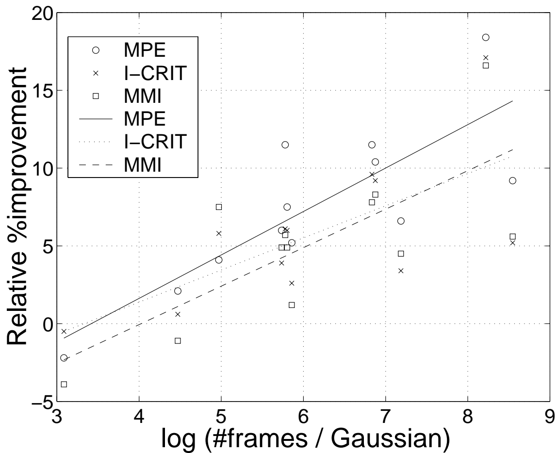
Figure 8.2: Relative improvement from MPE, I-Crit (I-smoothed MMI) and MMI on various corpora and setups, plotted against the \log_e(\#\text{frames}/\text{Gaussian}) of training data.
